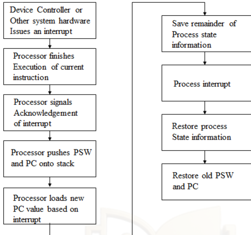
Fig: Simple Interrupt Processing
